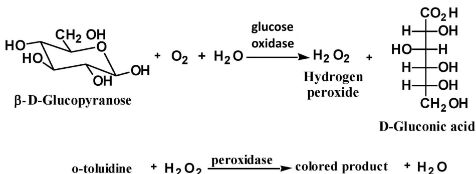
Figure 2. Reactions involved in the glucose oxidase/peroxidase kit containing o-toluidine and FDC yellow dye.
